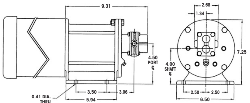
Close-Coupled: 33F-MC & 33F Sealed
