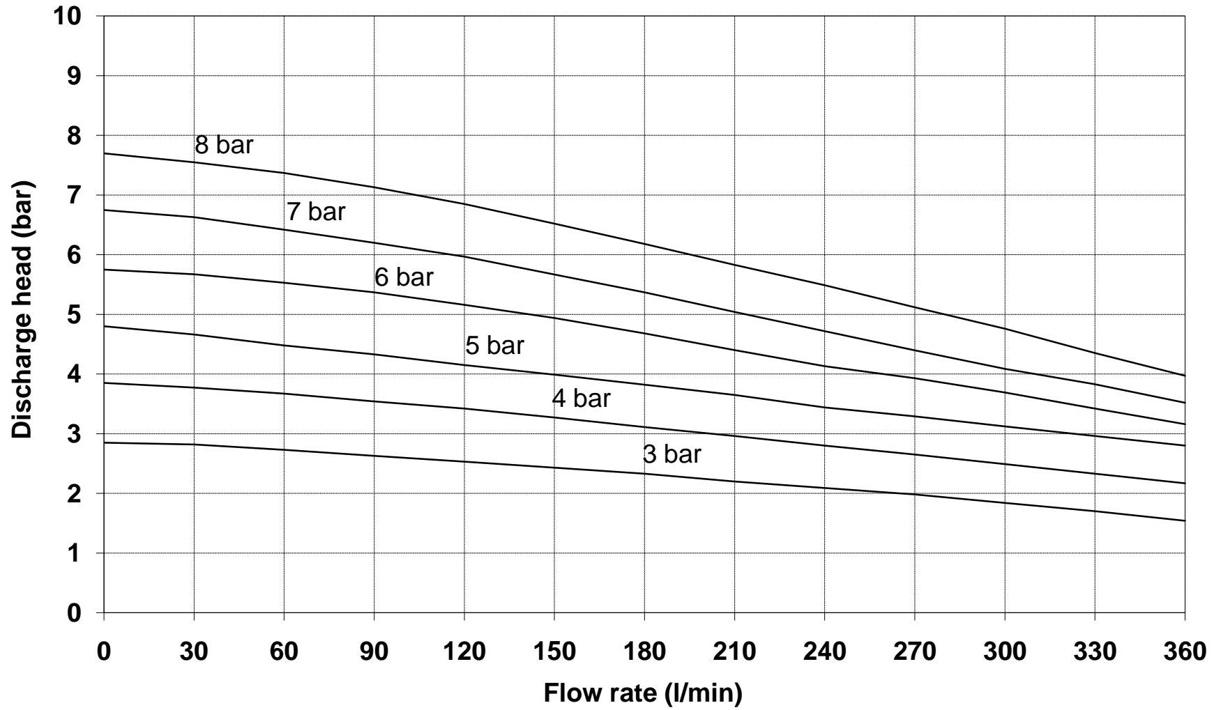
Performance curves/Model RP 150Duplex
