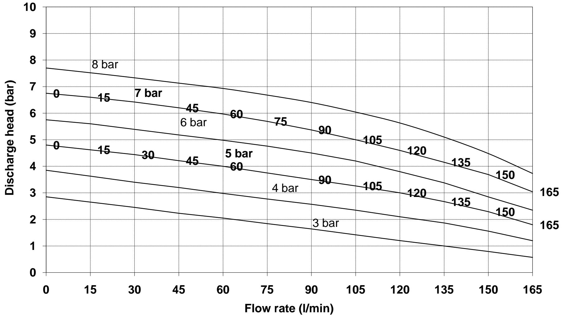
Performance curves/Model RP 150
