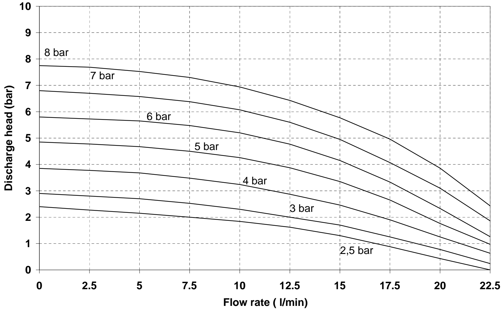
Performance Curves/ Model RP 20
