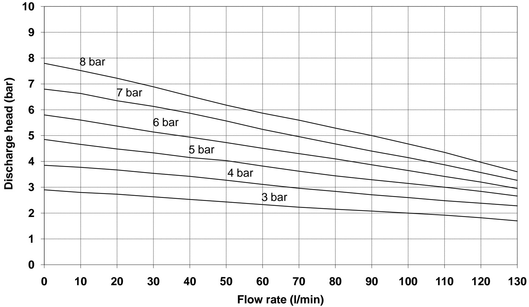
Performance curves/Model RP 60 Duplex
