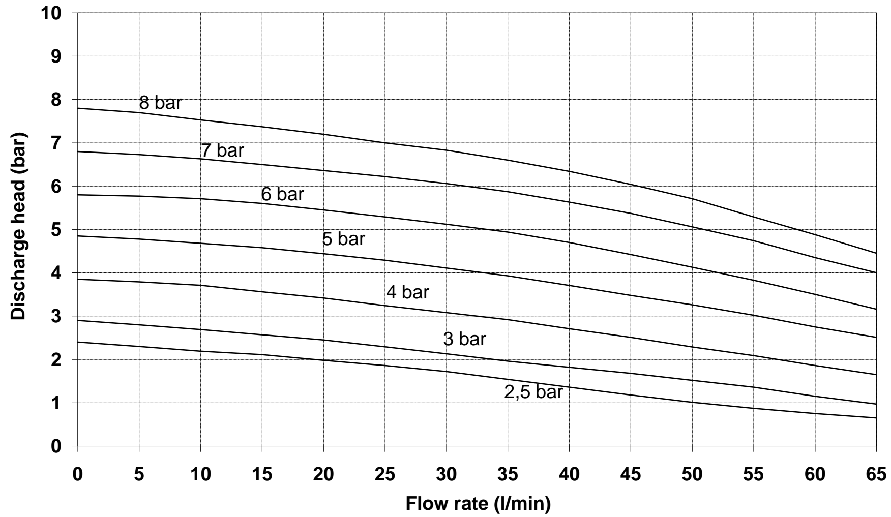
Performance curves/ Model RP 60
