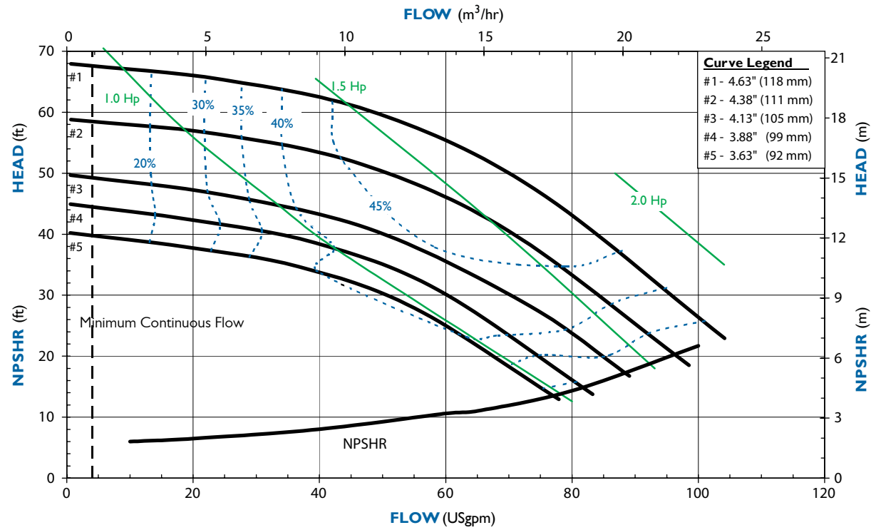
SP11 PERFORMANCE - Flooded Suction - 3450 RPM
