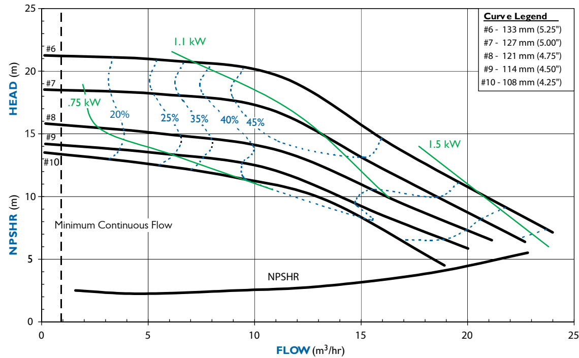
SP11 PERFORMANCE - Flooded Suction - 2900 RPM
