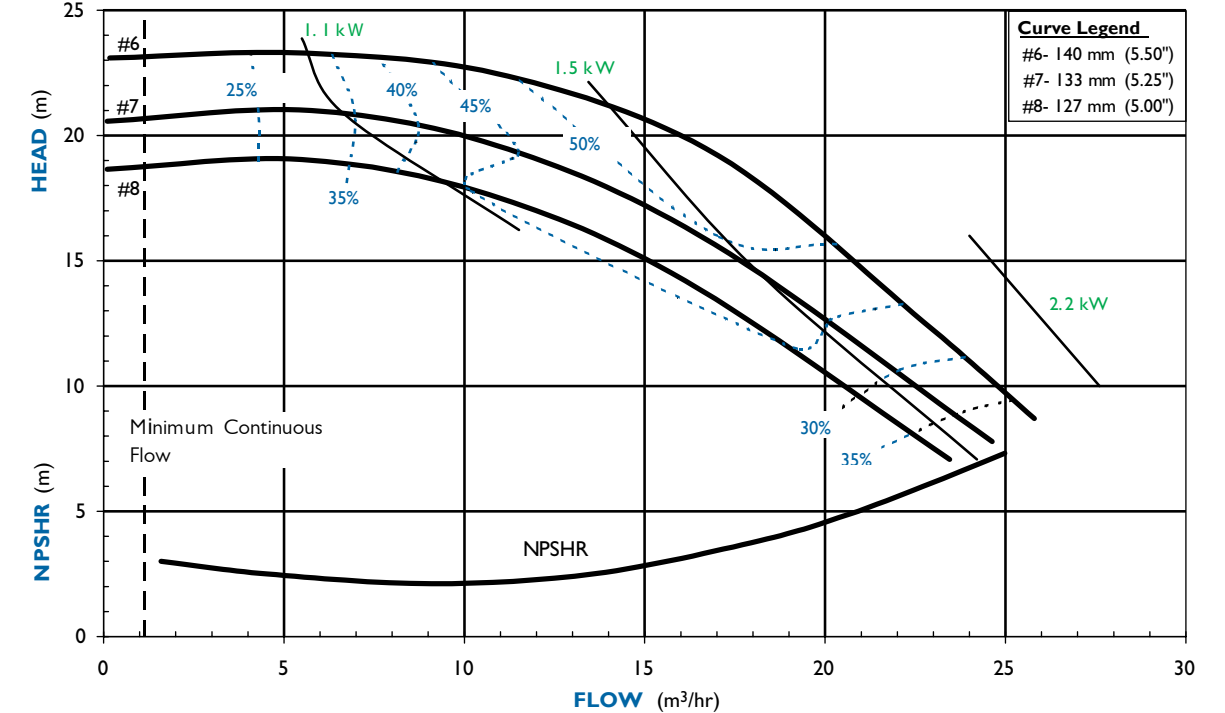
SP15 PERFORMANCE - Flooded Suction - 2900 RPM
