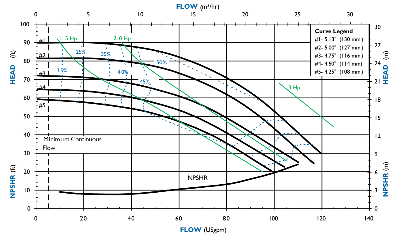
SP15 PERFORMANCE - Flooded Suction - 3450 RPM
