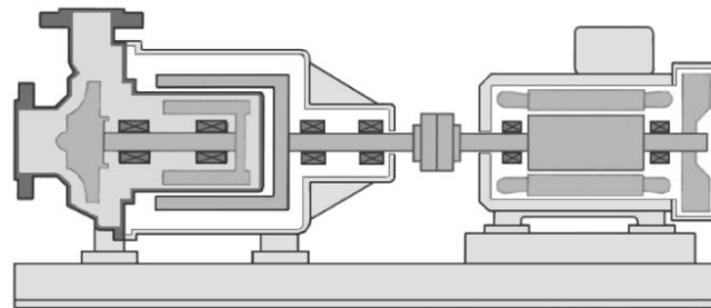
Centrifugal pump with magnet drive (end coupled)
