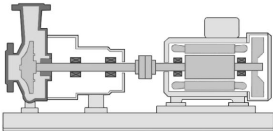
Centrifugal pump with shaft seal
