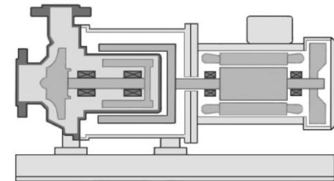
Centrifugal pump with magnet drive (close coupled)
