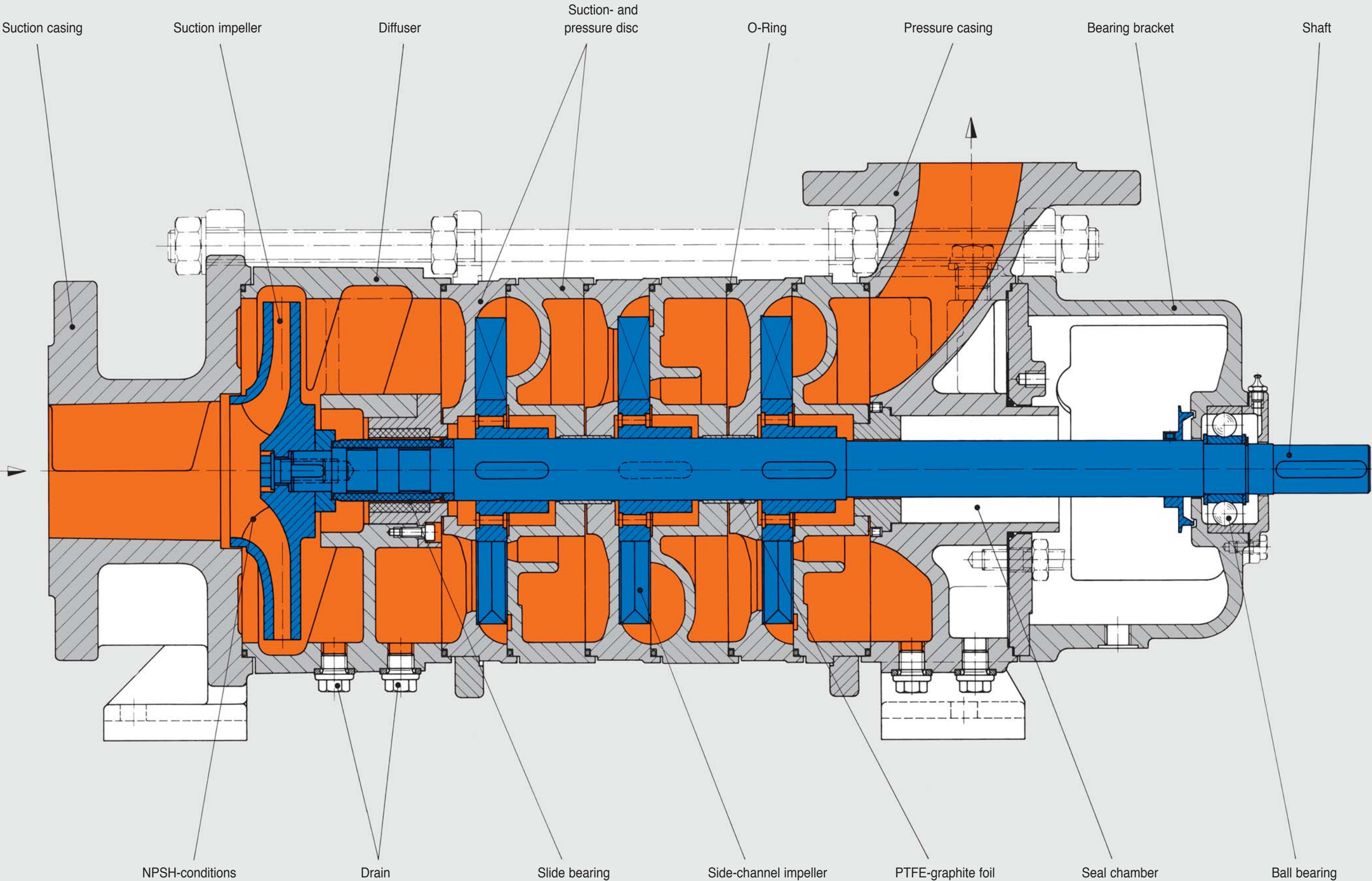
Sectional drawing
