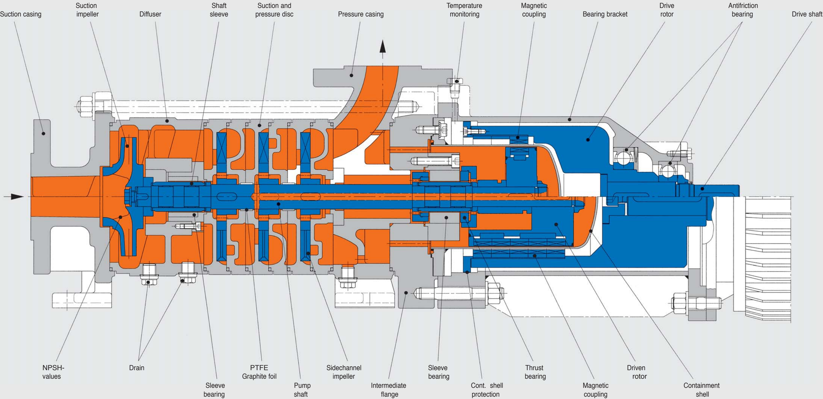
Sectional drawing
