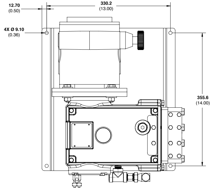
Metallic Pump Heads ATEX Zone 2 with Manual Adjustment
