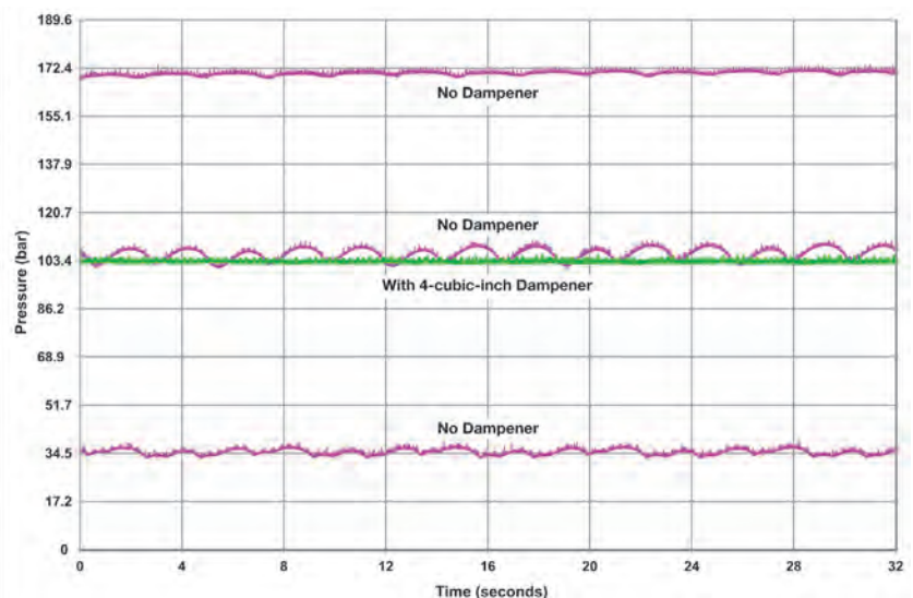
Hydra-Cell P500 Pressure Trace
