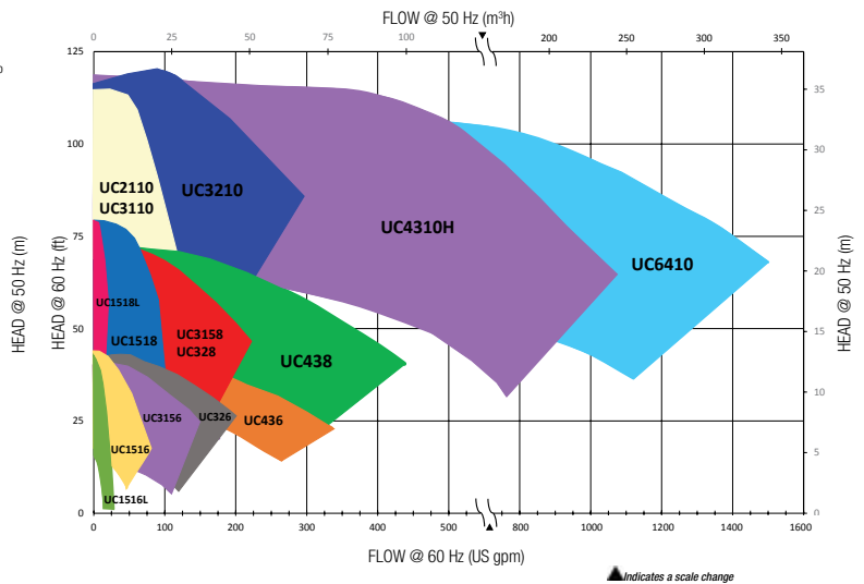
UC 4-Pole Coverage Chart
