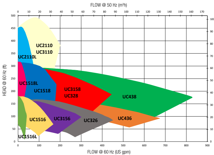
UC 2-Pole Coverage Chart
